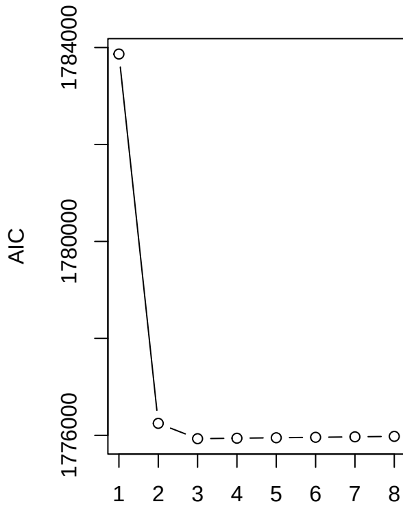
AIC
